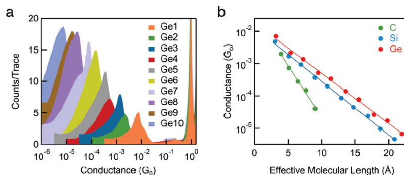
Figure 2. (a) Logarithm-binned 1D conductance histograms of Ge1–Ge10, each comprising thousands of measurement traces. (b) Conductance peak positions from the simple elongation measurements of C4–C8, Si1–Si10, and Ge1–Ge10 (panel a) plotted against effective molecular length ( L , in Å) give the decay constant \beta . \beta_{\text{C}} = 0.74 \pm 0.03 \text{ \AA}^{-1} , \beta_{\text{Si}} = 0.39 \pm 0.01 \text{ \AA}^{-1} , and \beta_{\text{Ge}} = 0.36 \pm 0.01 \text{ \AA}^{-1} .
